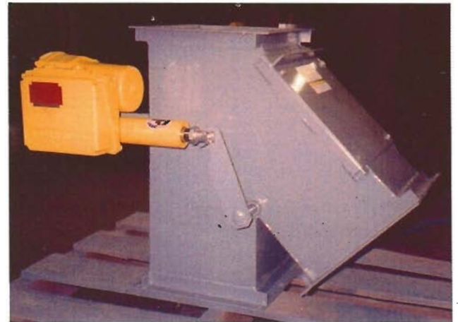
Automated "K" valve using electric actuator
