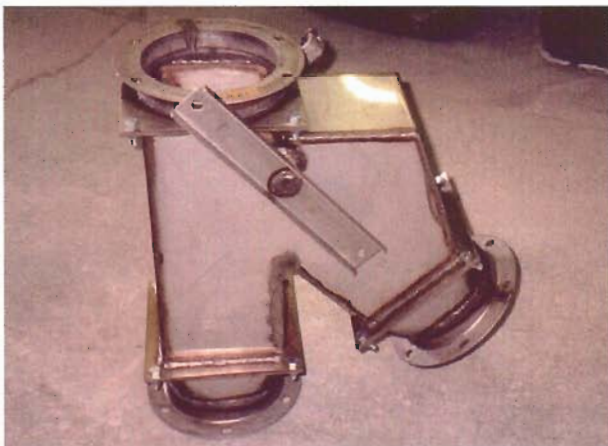
Stainless steel off set valve with flanged transitions
