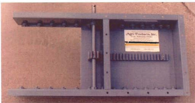
Roller type rack and pinion gate, heavy duty cast iron rack and pinion
