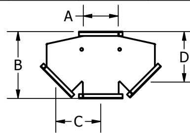
ELBOW SECTION
